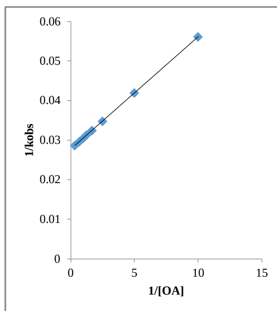
Figure 2. Oxidation of OA acid by TPACC: A double reciprocal plot
