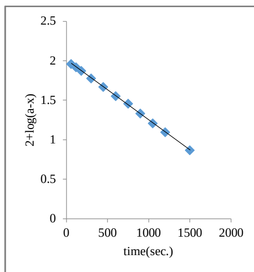
Oxidation of OA acid by TPACC: A typical kinetic run.
