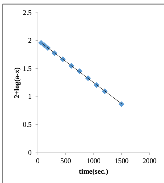
Figure 1. Oxidation of OA acid by TPACC: A typical kinetic run
